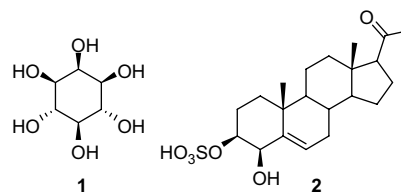
Figure 1. Samples for cyclitol and sulfate monoester.
