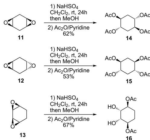
Scheme 4. Ring opening of syn - and anti -bisepoxides 11–13 and obtained products 14–16 .
