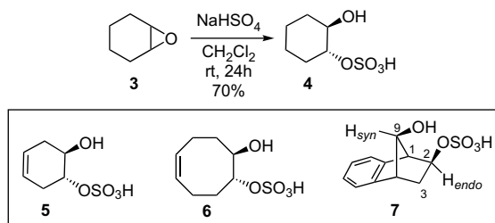
Scheme 1. Ring opening of epoxides with \text{NaHSO}_4 : obtained hydroxy sulfate ester.
